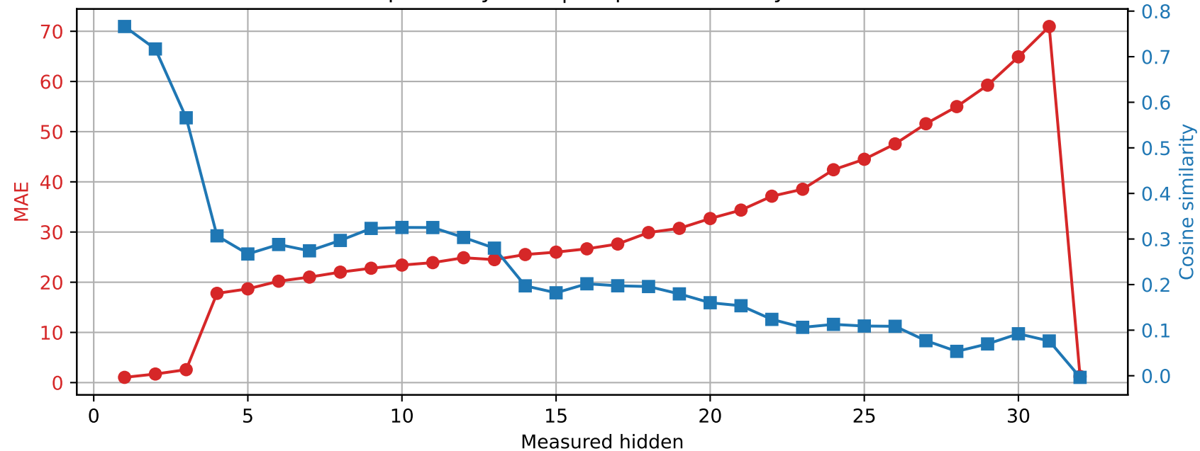
SmolLM2-360M | Prompt 0 Spared layer 12 | Unquantized vs hybrid
