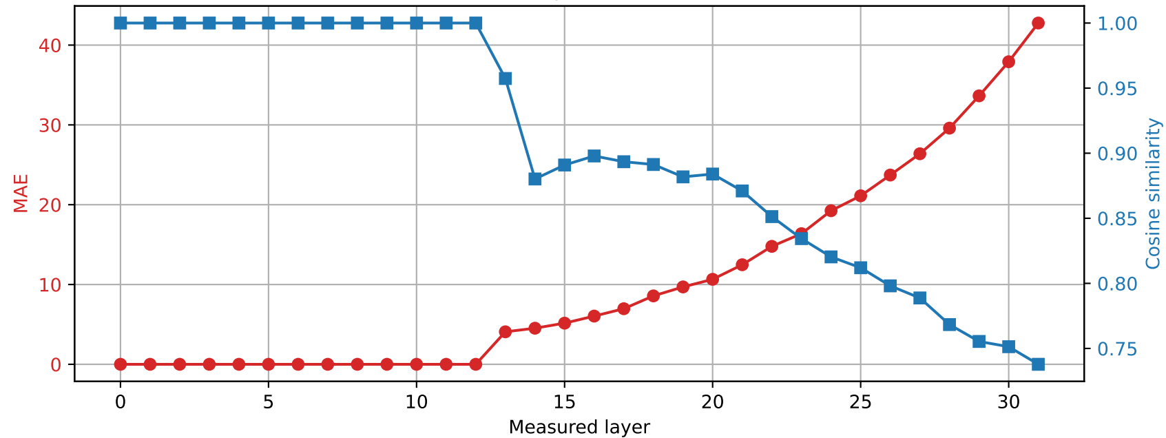
SmolLM2-360M | Prompt 0 Spared layer 12 | Hybrid vs quantized
