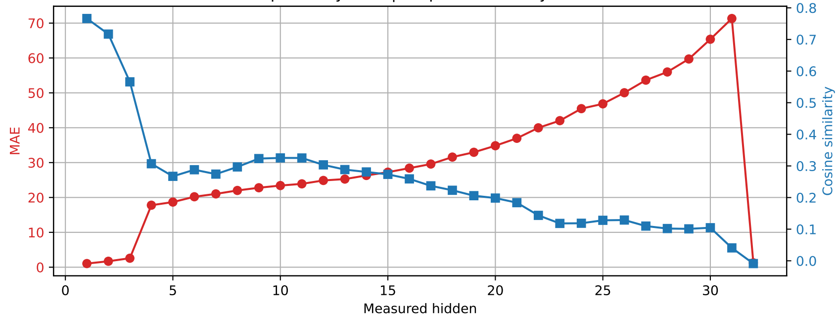
SmolLM2-360M | Prompt 0 Spared layer 17 | Unquantized vs hybrid
