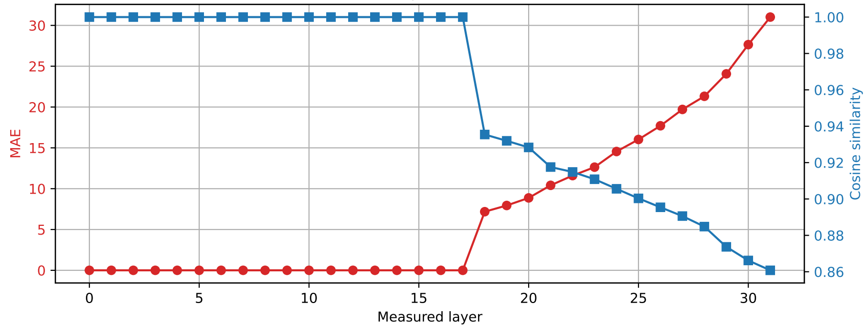
SmolLM2-360M | Prompt 0 Spared layer 17 | Hybrid vs quantized
