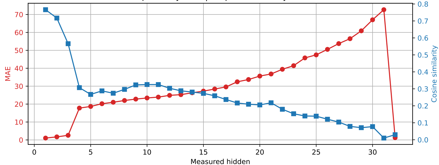
SmolLM2-360M | Prompt 0 Spared layer 20 | Unquantized vs hybrid
