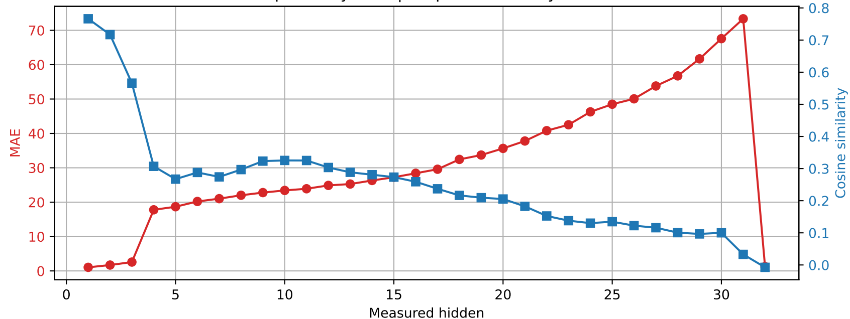
SmolLM2-360M | Prompt 0 Spared layer 25 | Unquantized vs hybrid
