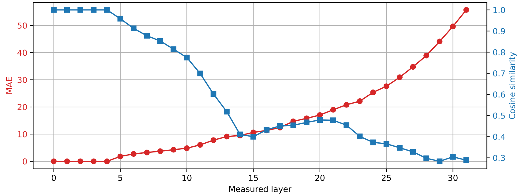
SmolLM2-360M | Prompt 1 Spared layer 4 | Hybrid vs quantized
