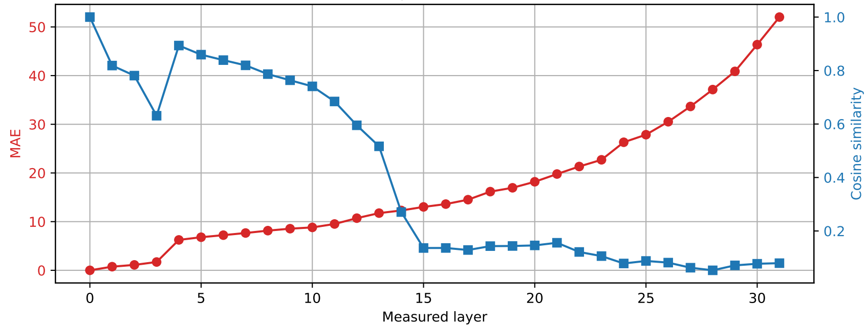
SmolLM2-360M | Prompt 1 Spared layer 4 | Hybrid vs unquantized
