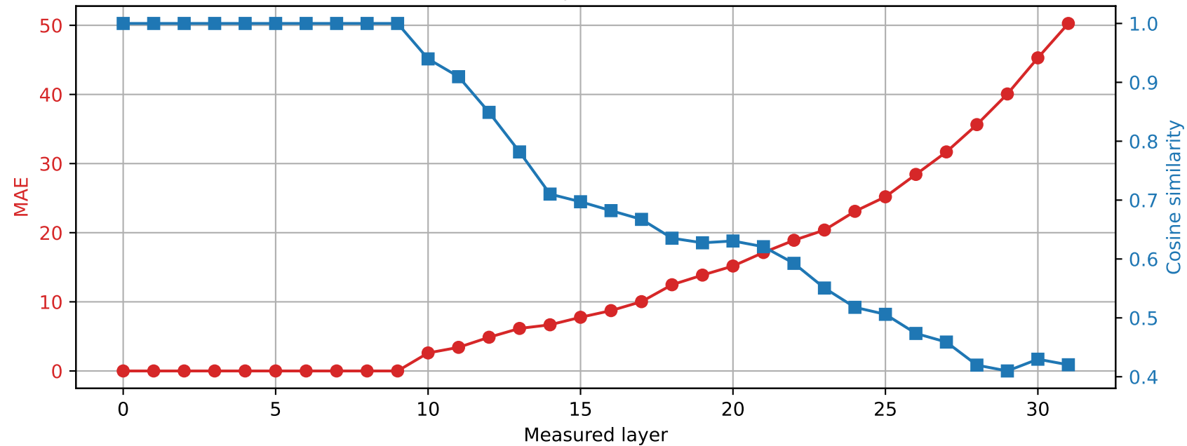
SmolLM2-360M | Prompt 1 Spared layer 9 | Hybrid vs quantized
