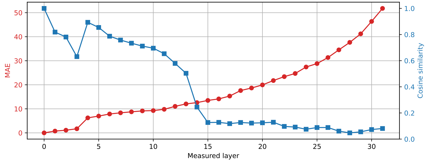
SmolLM2-360M | Prompt 1 Spared layer 9 | Hybrid vs unquantized
