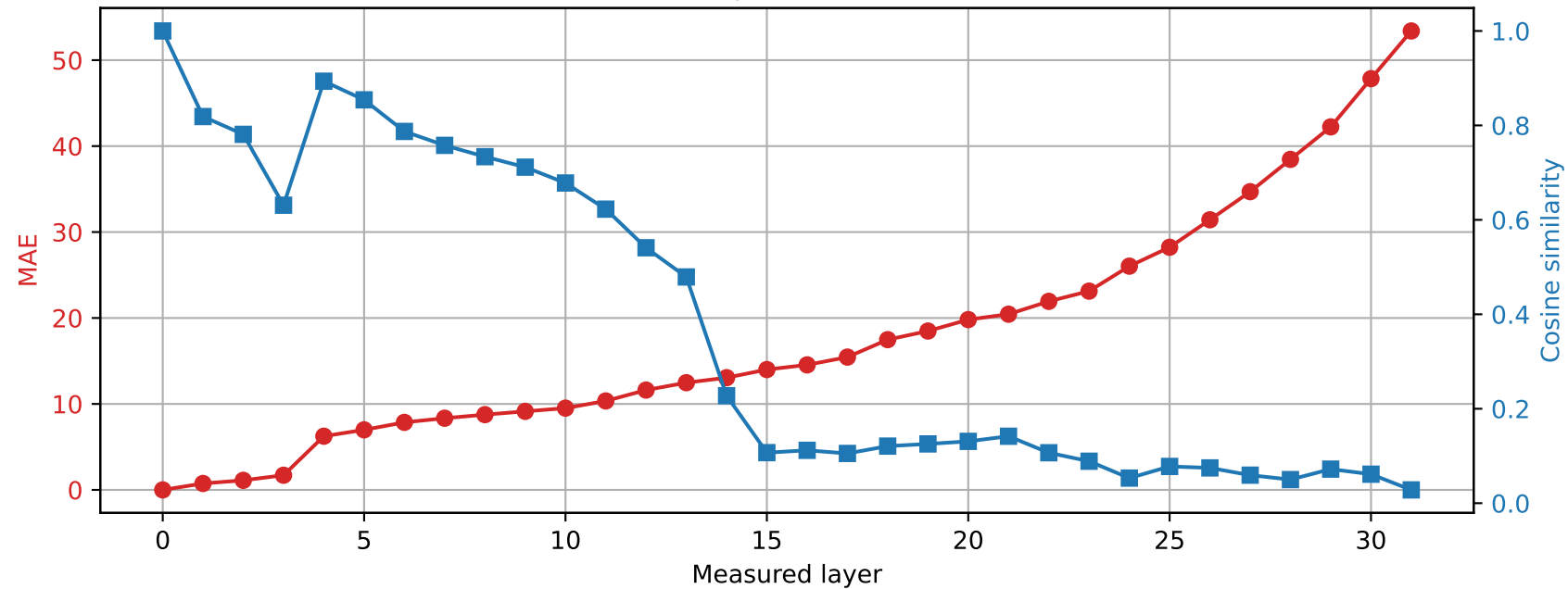
SmolLM2-360M | Prompt 1 Spared layer 20 | Hybrid vs unquantized
