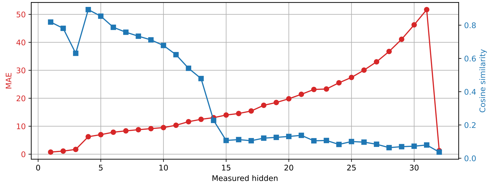
SmolLM2-360M | Prompt 1 Spared layer 22 | Unquantized vs hybrid
