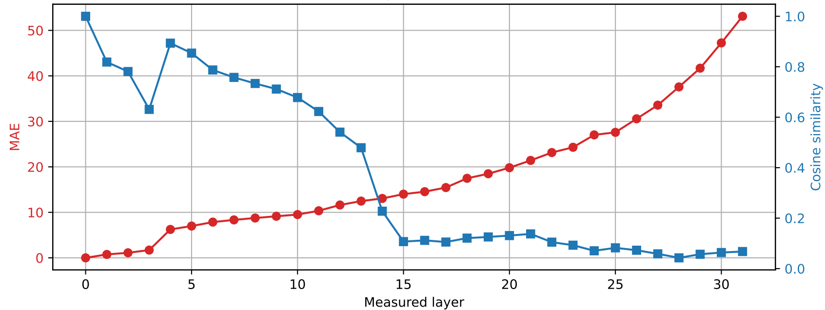
SmolLM2-360M | Prompt 1 Spared layer 24 | Hybrid vs unquantized
