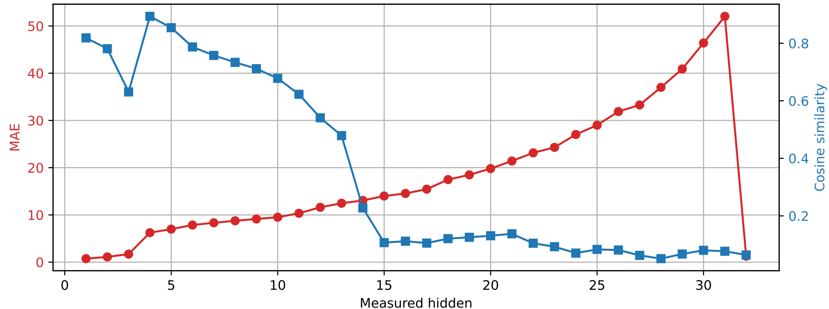
SmolLM2-360M | Prompt 1 Spared layer 26 | Unquantized vs hybrid
