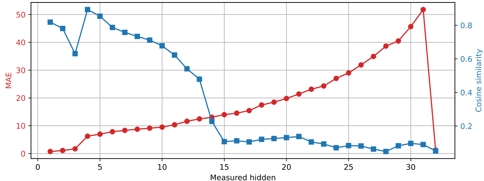
SmolLM2-360M | Prompt 1 Spared layer 28 | Unquantized vs hybrid
