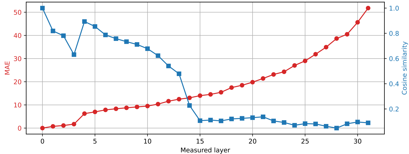
SmolLM2-360M | Prompt 1 Spared layer 28 | Hybrid vs unquantized
