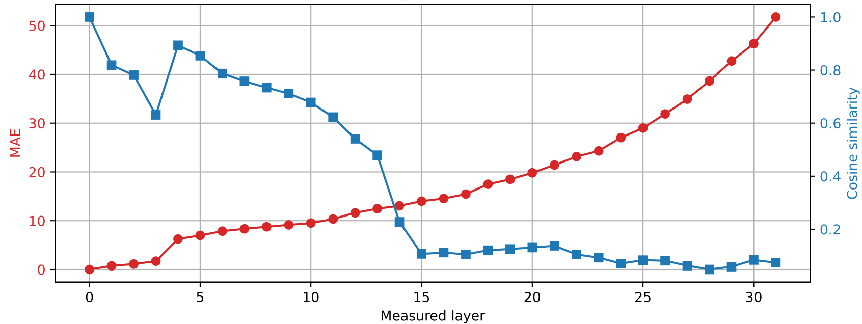
SmolLM2-360M | Prompt 1 Spared layer 29 | Hybrid vs unquantized
