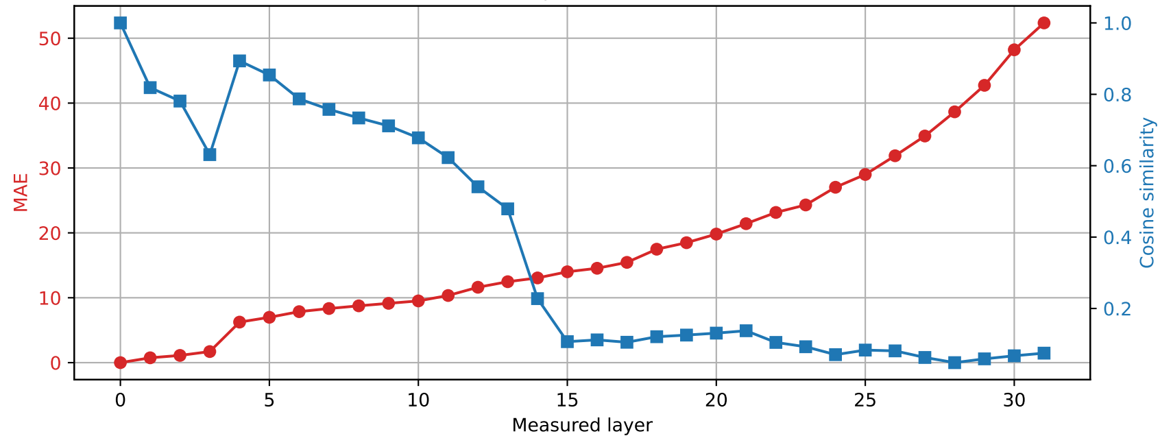
SmolLM2-360M | Prompt 1 Spared layer 30 | Hybrid vs unquantized
