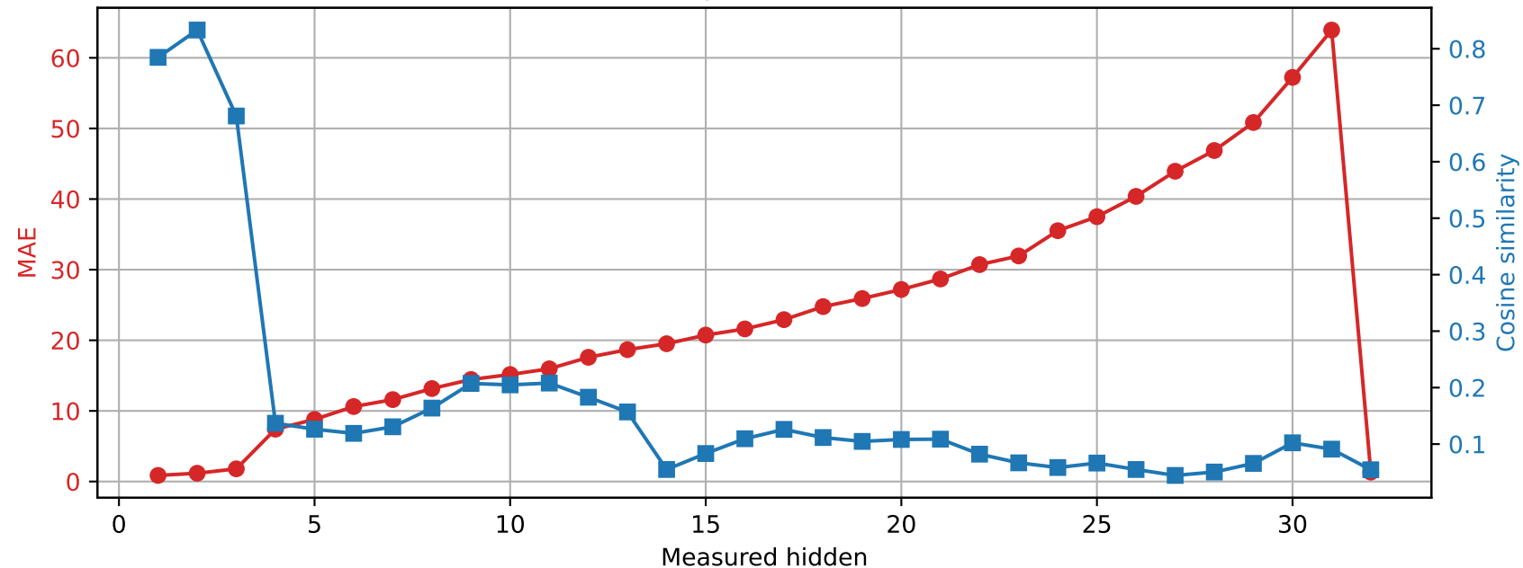
SmolLM2-360M | Prompt 2 Spared layer 1 | Unquantized vs hybrid
