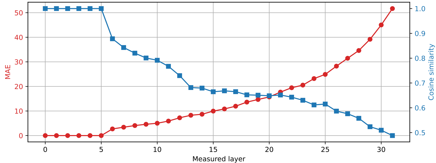
SmolLM2-360M | Prompt 2 Spared layer 5 | Hybrid vs quantized
