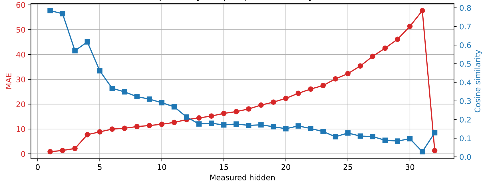
SmolLM2-360M | Prompt 2 Spared layer 6 | Unquantized vs hybrid
