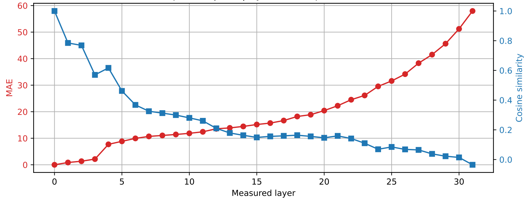
SmolLM2-360M | Prompt 2 Spared layer 7 | Hybrid vs unquantized
