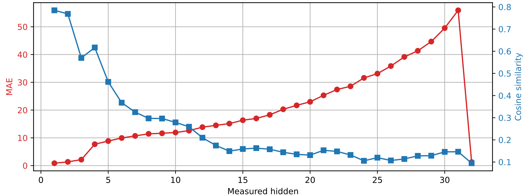
SmolLM2-360M | Prompt 2 Spared layer 8 | Unquantized vs hybrid
