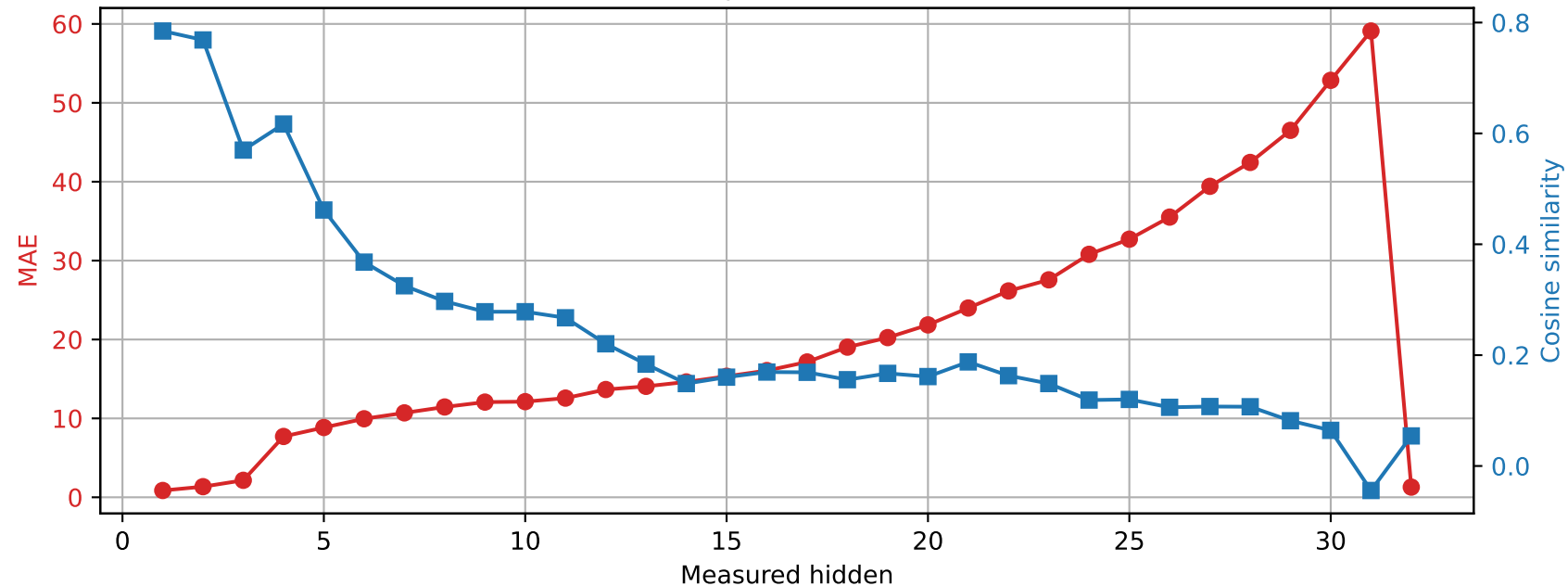
SmolLM2-360M | Prompt 2 Spared layer 9 | Unquantized vs hybrid
