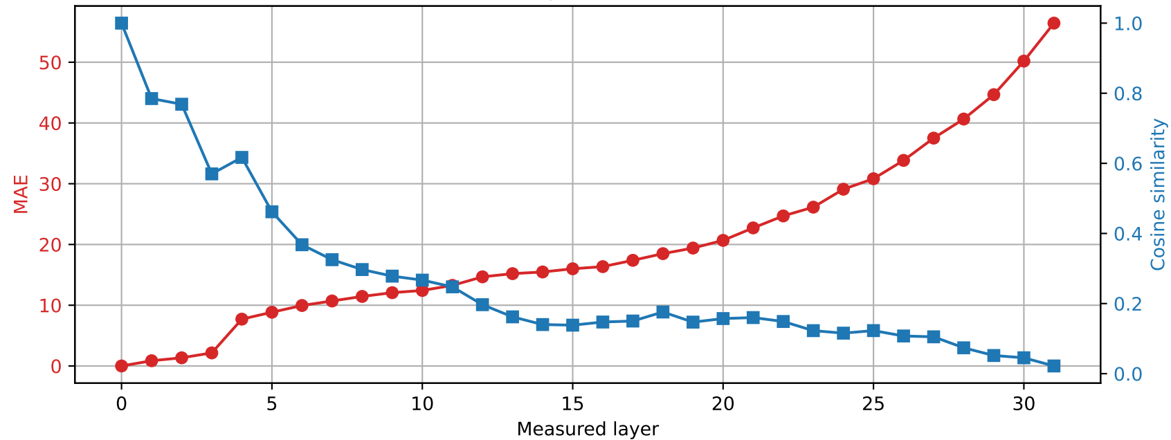
SmolLM2-360M | Prompt 2 Spared layer 13 | Hybrid vs unquantized
