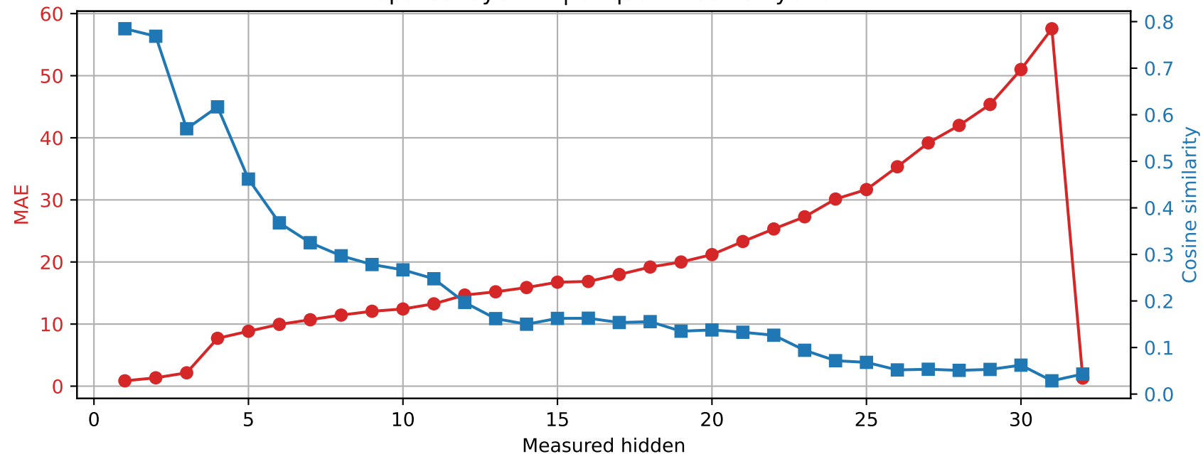
SmolLM2-360M | Prompt 2 Spared layer 14 | Unquantized vs hybrid
