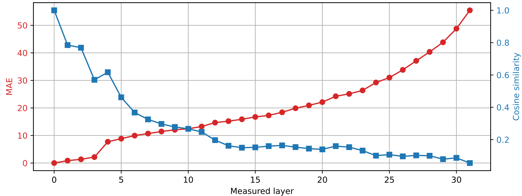
SmolLM2-360M | Prompt 2 Spared layer 21 | Hybrid vs unquantized
