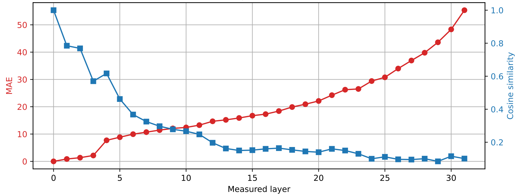
SmolLM2-360M | Prompt 2 Spared layer 22 | Hybrid vs unquantized
