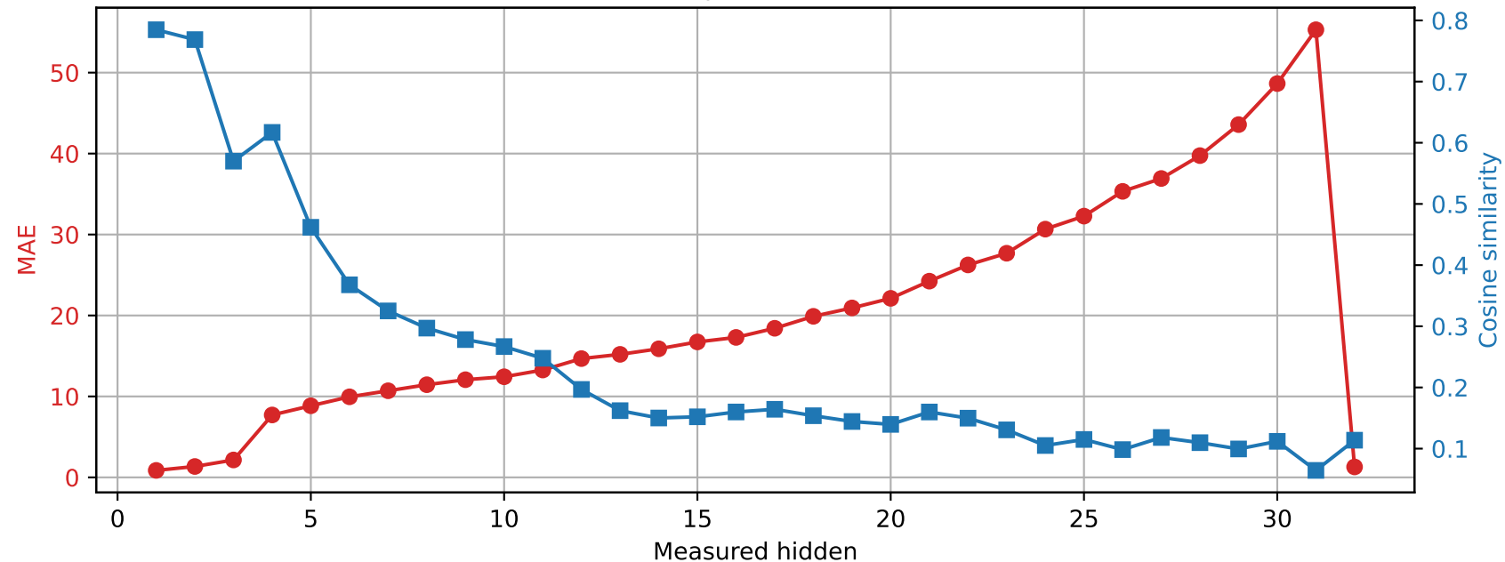
SmolLM2-360M | Prompt 2 Spared layer 26 | Unquantized vs hybrid
