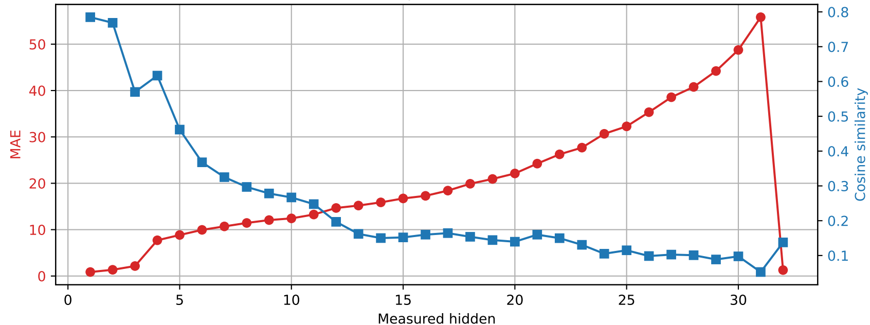
SmolLM2-360M | Prompt 2 Spared layer 27 | Unquantized vs hybrid
