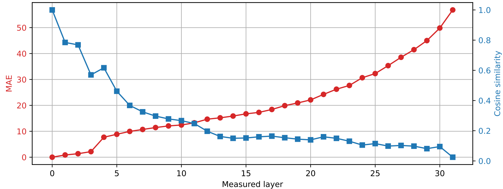
SmolLM2-360M | Prompt 2 Spared layer 31 | Hybrid vs unquantized
