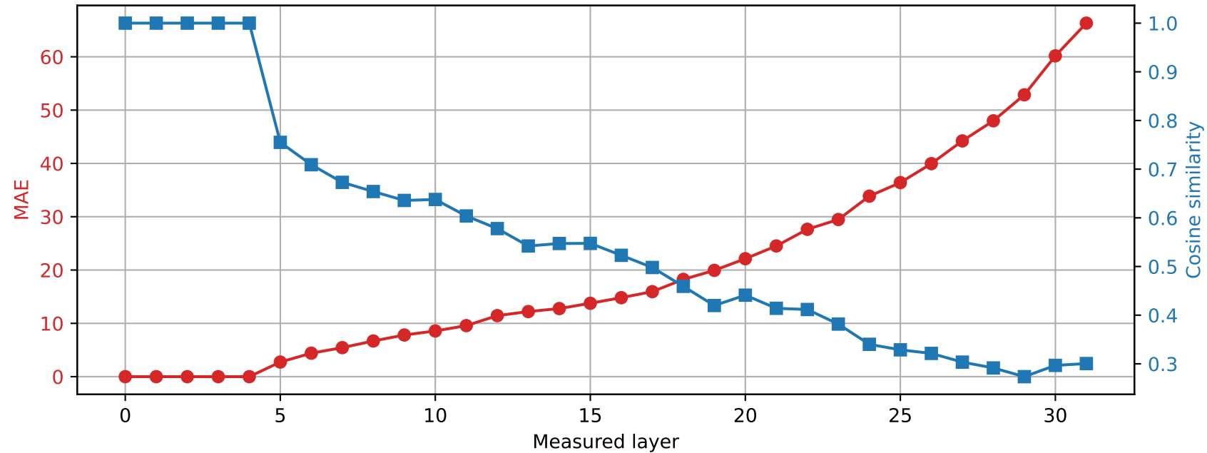
SmolLM2-360M | Prompt 3 Spared layer 4 | Hybrid vs quantized
