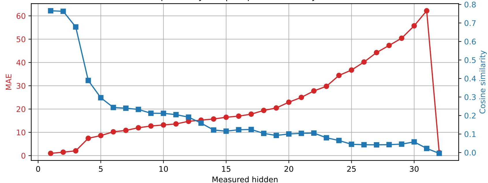
SmolLM2-360M | Prompt 3 Spared layer 6 | Unquantized vs hybrid
