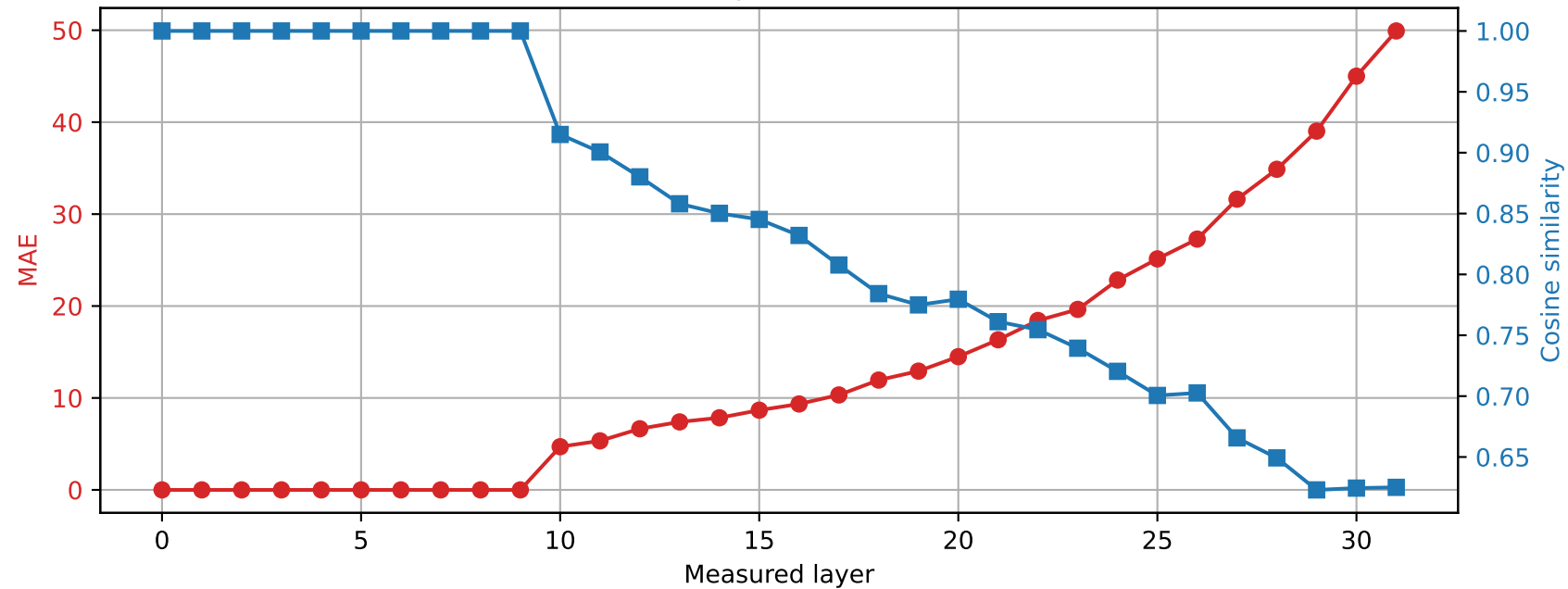
SmolLM2-360M | Prompt 3 Spared layer 9 | Hybrid vs quantized
