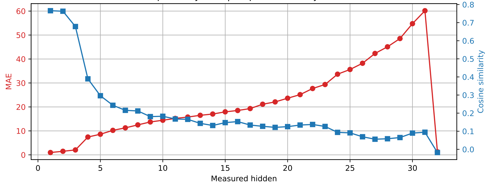
SmolLM2-360M | Prompt 3 Spared layer 11 | Unquantized vs hybrid
