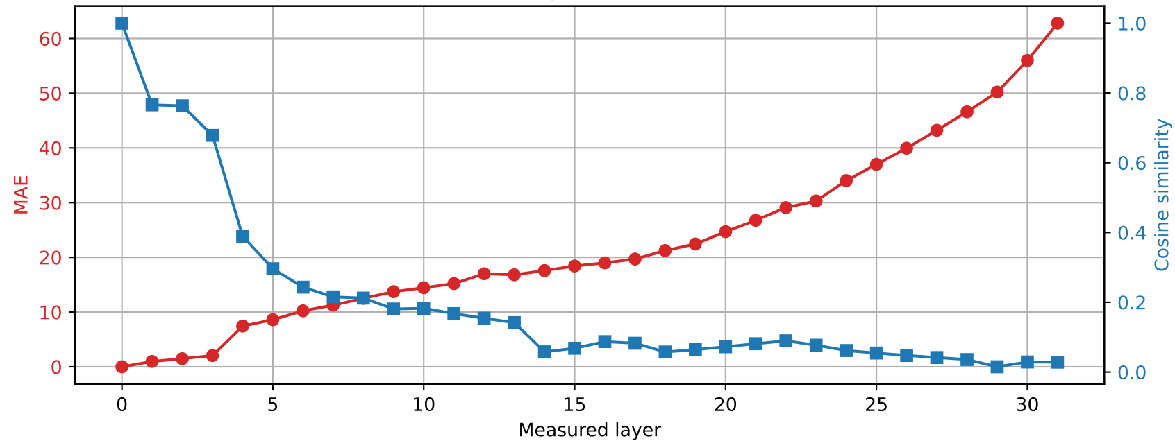
SmolLM2-360M | Prompt 3 Spared layer 12 | Hybrid vs unquantized
