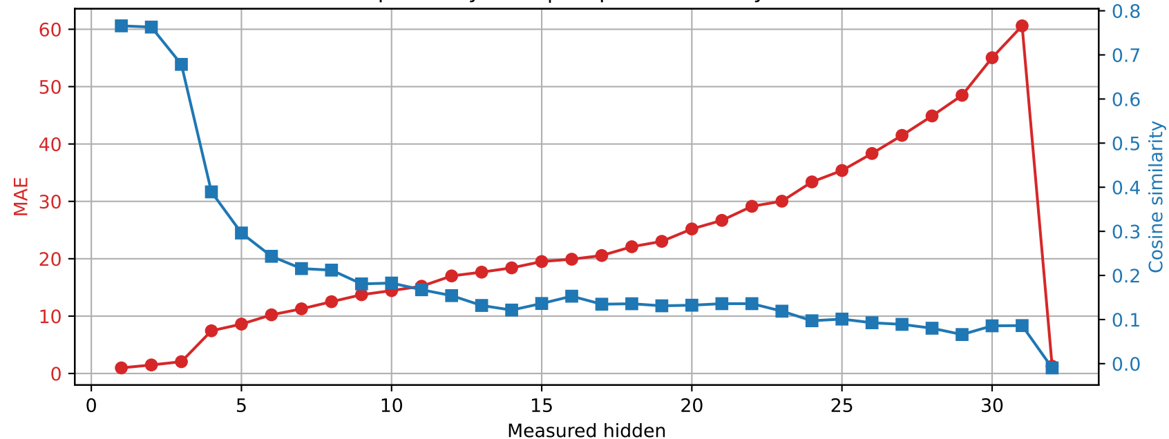
SmolLM2-360M | Prompt 3 Spared layer 14 | Unquantized vs hybrid
