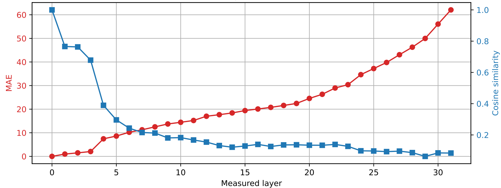
SmolLM2-360M | Prompt 3 Spared layer 17 | Hybrid vs unquantized
