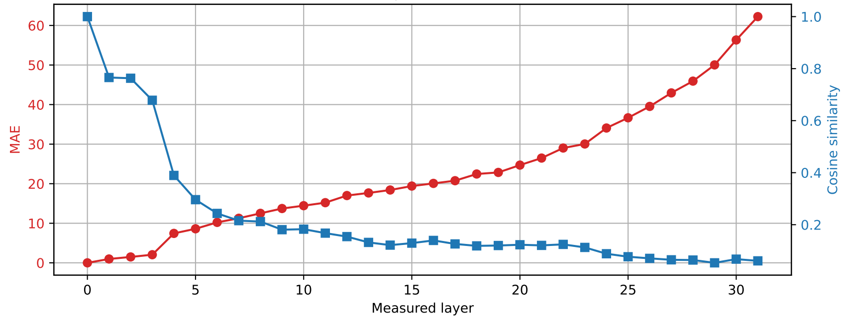
SmolLM2-360M | Prompt 3 Spared layer 18 | Hybrid vs unquantized
