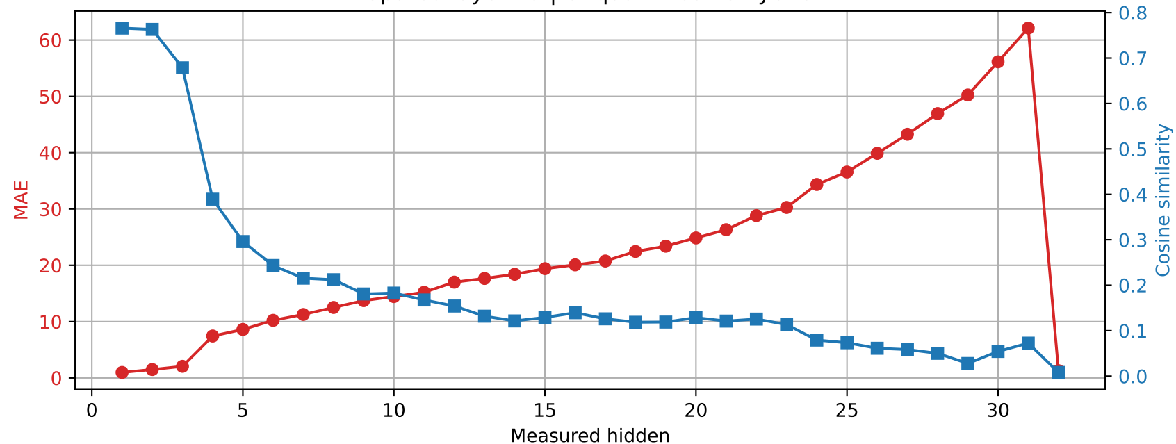
SmolLM2-360M | Prompt 3 Spared layer 19 | Unquantized vs hybrid
