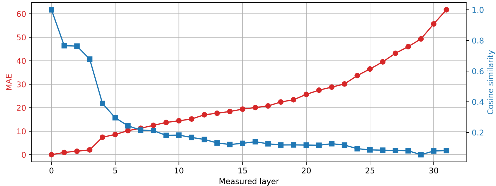
SmolLM2-360M | Prompt 3 Spared layer 21 | Hybrid vs unquantized
