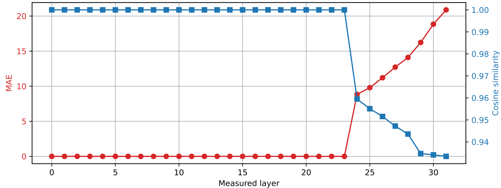
SmolLM2-360M | Prompt 3 Spared layer 23 | Hybrid vs quantized
