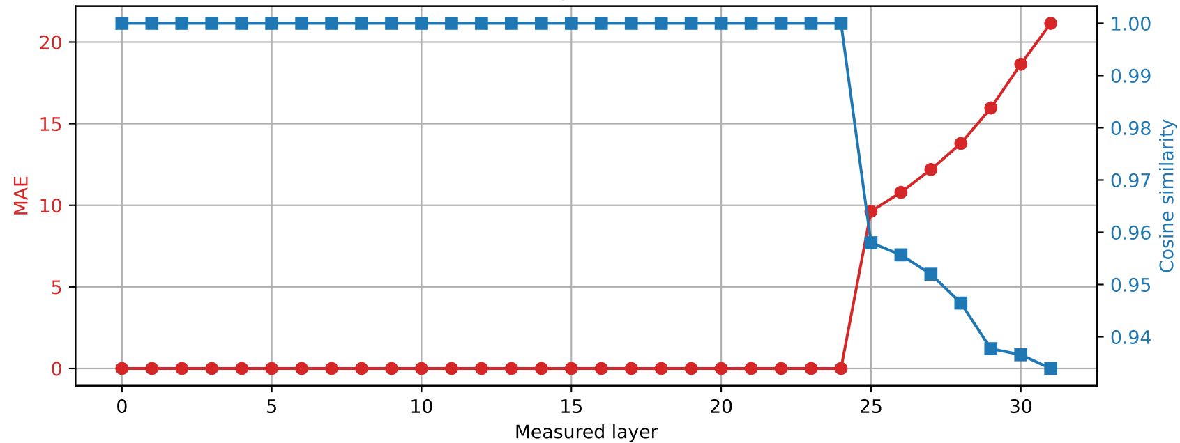
SmolLM2-360M | Prompt 3 Spared layer 24 | Hybrid vs quantized
