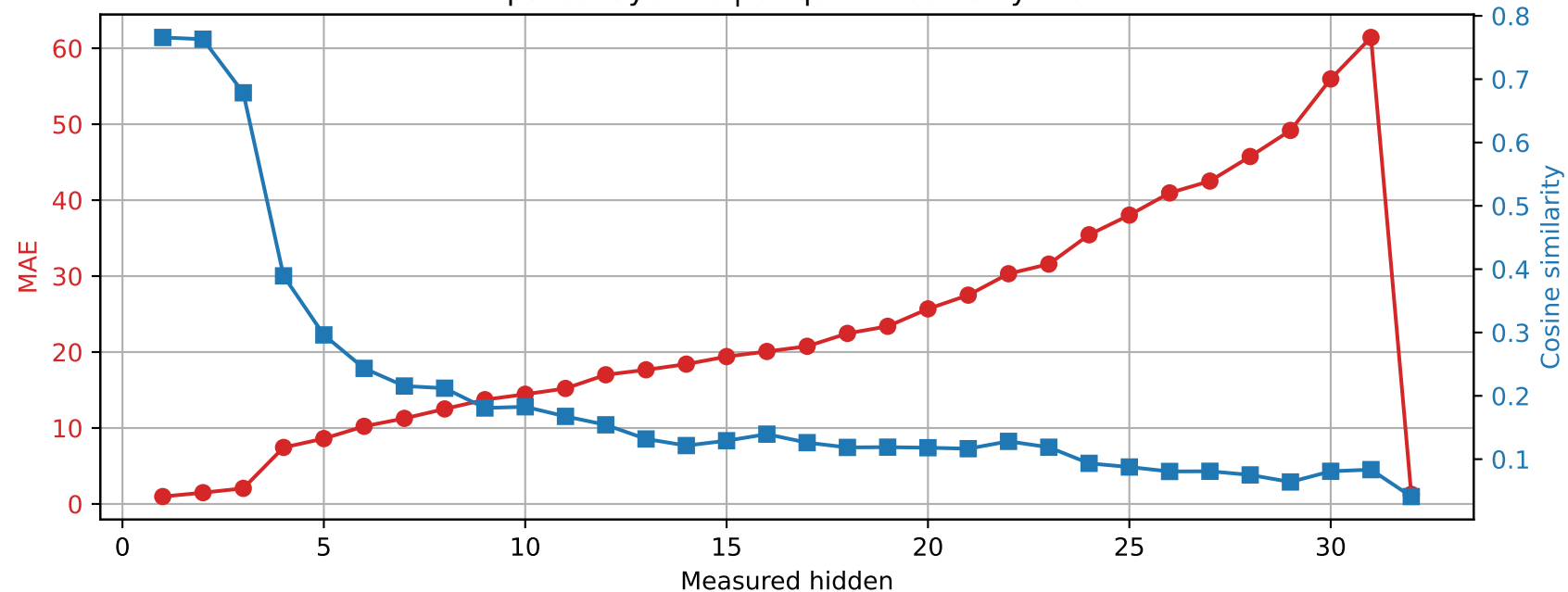
SmolLM2-360M | Prompt 3 Spared layer 26 | Unquantized vs hybrid
