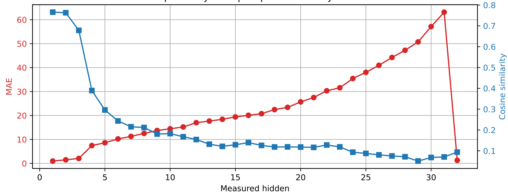
SmolLM2-360M | Prompt 3 Spared layer 31 | Unquantized vs hybrid
