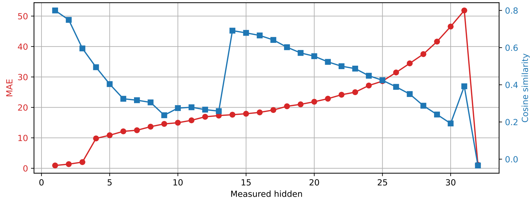
SmolLM2-360M | Prompt 4 Spared layer 6 | Unquantized vs hybrid
