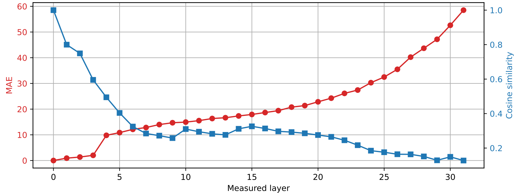
SmolLM2-360M | Prompt 4 Spared layer 8 | Hybrid vs unquantized
