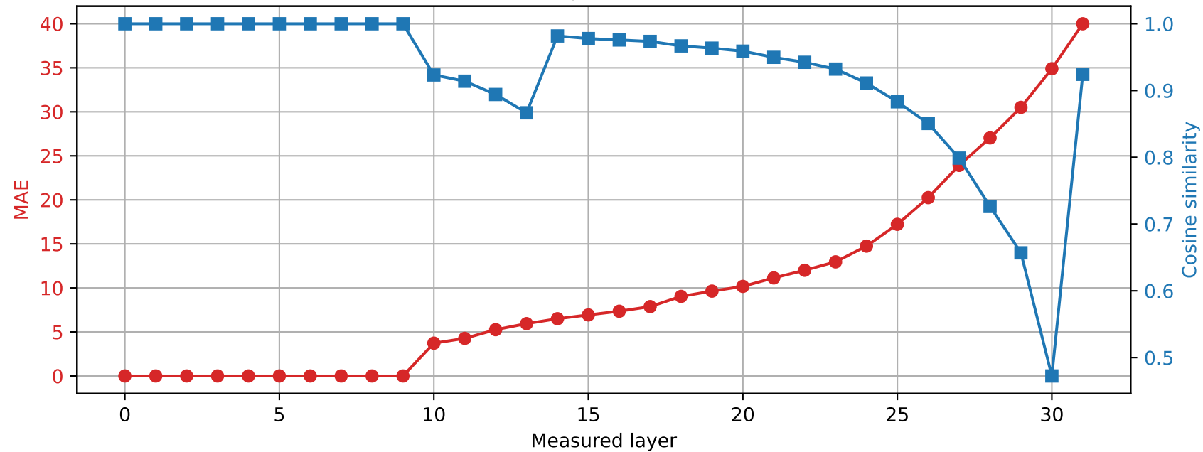
SmolLM2-360M | Prompt 4 Spared layer 9 | Hybrid vs quantized
