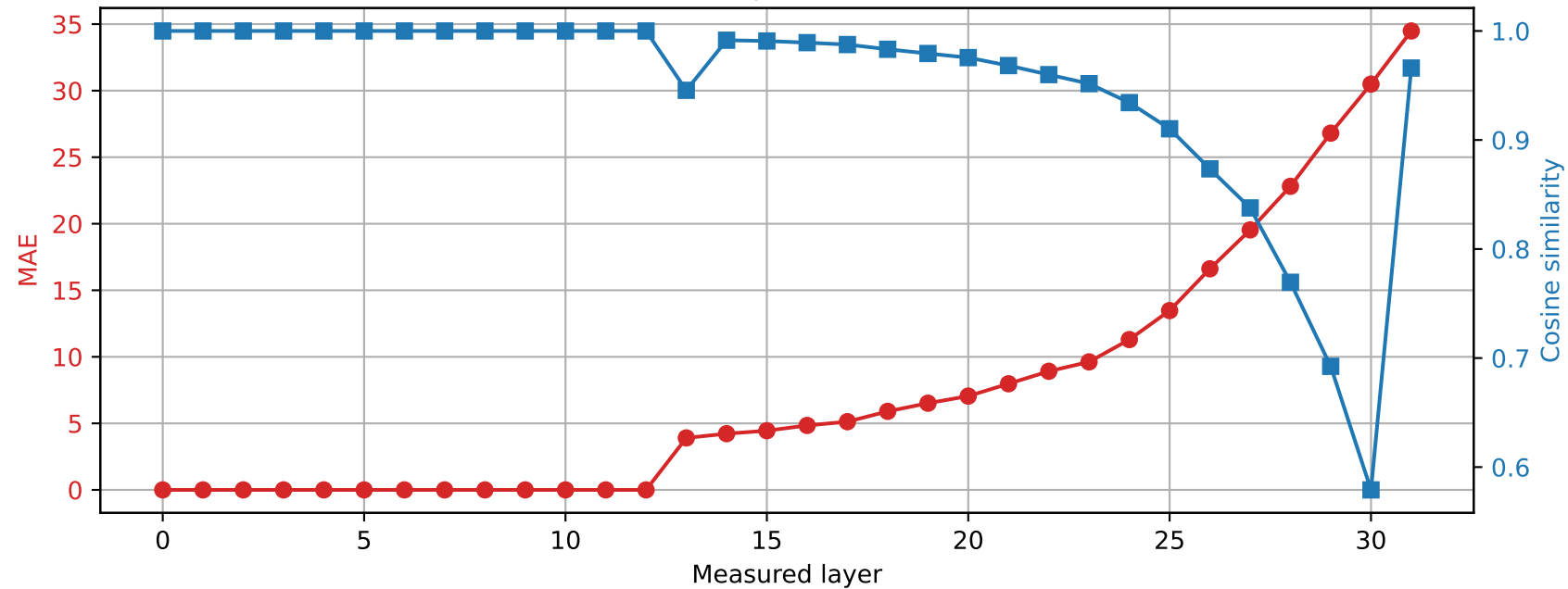
SmolLM2-360M | Prompt 4 Spared layer 12 | Hybrid vs quantized
