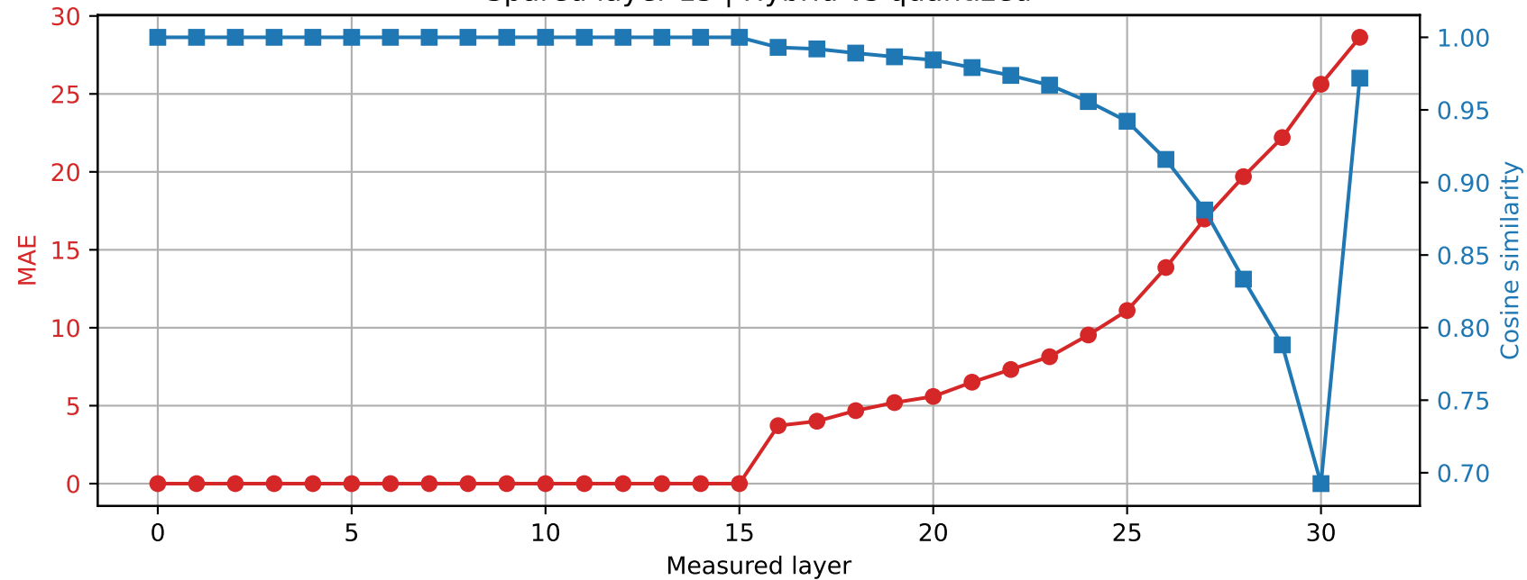
SmolLM2-360M | Prompt 4 Spared layer 15 | Hybrid vs quantized
